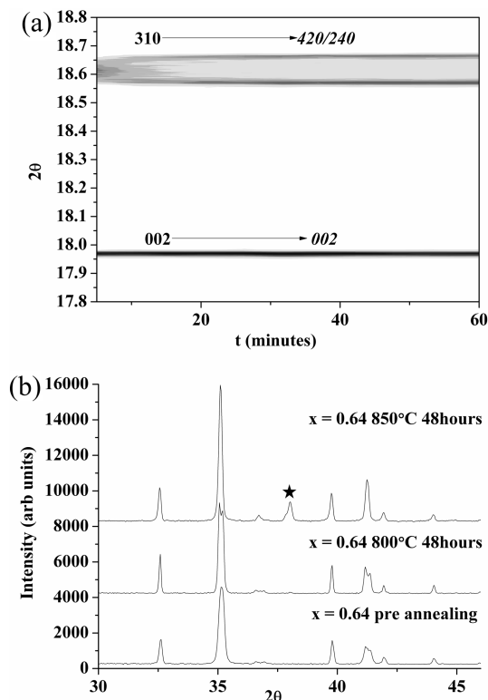
Figure 6. (a) Diffraction from \text{La}_{1.64}\text{Sr}_{0.36}\text{Ga}_3\text{O}_{7.32} at 400 °C showing the transition from metastable T to stable O phase. T Miller indices in bold and O in italics. (b) XRD patterns of \text{La}_{1.64}\text{Sr}_{0.36}\text{Ga}_3\text{O}_{7.32} before annealing, after annealing at 800 °C for 48 h, and after 850 °C for 48 h. The black star shows the formation of strontium doped lanthanum gallate (LSG) perovskite.
