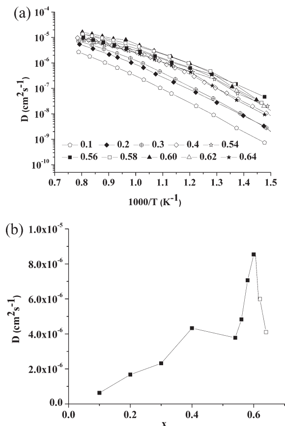
Figure 11. (a) Diffusion coefficients of \text{La}_{1+x}\text{Sr}_{1-x}\text{Ga}_3\text{O}_{7+x/2} ( x = 0\text{--}0.64 ). (b) Diffusion coefficient versus x at 800 °C.
