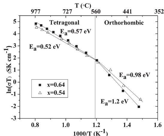
Figure 8. Conductivity of \text{La}_{1.64}\text{Sr}_{0.36}\text{Ga}_3\text{O}_{7.32} (black squares, T at high temperature, O at low temperature) and \text{La}_{1.54}\text{Sr}_{0.46}\text{Ga}_3\text{O}_{7.27} (triangles, T at all temperatures). The lines show the two regions with different activation energies. The postmeasurement XRD is given in SI Figure S5a.
