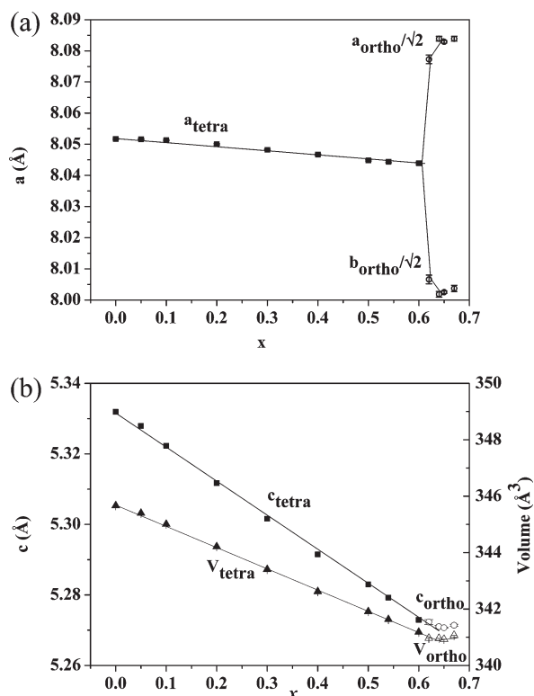
Figure 4. (a) a and b lattice parameters. (b) c parameter and unit cell volume of \text{La}_{1+x}\text{Sr}_{1-x}\text{Ga}_3\text{O}_{7+x/2} , x = 0-0.67 . Data for x < 0.6 are from ref 9; that for x > 0.6 is from this work.
