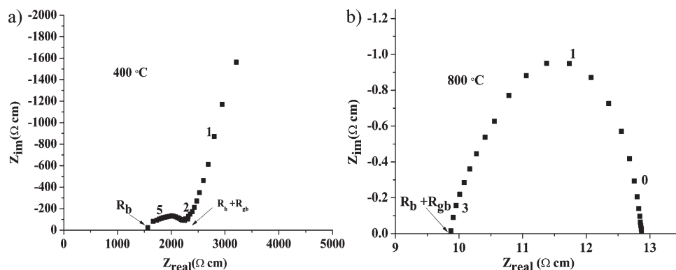
Figure 2. Complex impedance plots of \text{La}_{1.6}\text{Sr}_{0.4}\text{Ga}_3\text{O}_{7.3} at 400 (a) and 800 °C (b). The numbers in bold on the plot indicate the frequency logarithms; the ac amplitude used for the measurements was 10 mV.
