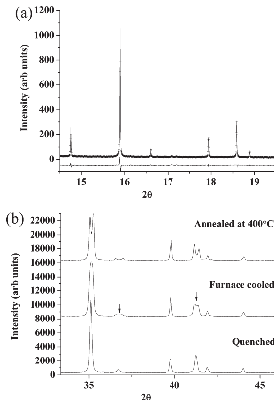
Figure 5. (a) LeBail fit of \text{La}_{1.64}\text{Sr}_{0.36}\text{Ga}_3\text{O}_{7.32} at 600 °C using the tetragonal space group P4_2/m ( \lambda = 0.825451 Å, R_{wp} = 7.965\% ). (b) \text{La}_{1.64}\text{Sr}_{0.36}\text{Ga}_3\text{O}_{7.32} after quenching, furnace cooling, and annealing for 12 h at 400 °C. The arrows indicate the tetragonal peaks in the pseudo-orthorhombic dominated furnace-cooled sample.
