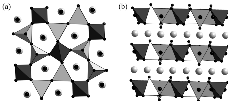
Figure 1. Melilite structure of LaSrGa 3 O 7 showing the two types of GaO 4 tetrahedra (dark gray 4-connected, light gray/white 3-connected). Light gray spheres show the La/Sr sites, and the black spheres show oxygen. The spheres for the interstitial oxygen sites are larger than those for the framework oxygens. In part a, the view is down the c axis showing the Ga tetrahedra and the pentagonal tunnels. The view in part b along [110] shows that the interstitial oxygen sits in the center of the Ga layers with La/Sr cations above and below.
