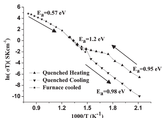
Figure 9. Conductivity of quenched \text{La}_{1.64}\text{Sr}_{0.36}\text{Ga}_3\text{O}_{7.32} during thermal cycling is given by triangles. Initially the sample is tetragonal converting to orthorhombic on heating above 400 °C; on cooling, this sample retains the orthorhombic structure. The conductivity of a second sample of \text{La}_{1.64}\text{Sr}_{0.36}\text{Ga}_3\text{O}_{7.32} which was furnace cooled from 1350 °C is also given for comparison and denoted by stars. This material adopts the tetragonal structure above 565 °C below which it reverts to the orthorhombic structure. Postmeasurement XRD of the furnace cooled sample (stars) is shown in SI Figure S5a; postmeasurement XRD of the quenched sample (triangles) is shown in Figure S5b.
