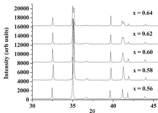
Figure 3. XRD patterns of \text{La}_{1+x}\text{Sr}_{1-x}\text{Ga}_3\text{O}_{7+x/2} ( x = 0.56, 0.58, 0.6, 0.62 , and 0.64 ).
