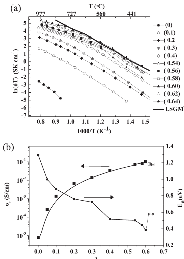
Figure 10. (a) Conductivity of \text{La}_{1+x}\text{Sr}_{1-x}\text{Ga}_3\text{O}_{7+x/2} where x = 0\text{--}0.64 . LSGM is \text{La}_{0.8}\text{Sr}_{0.2}\text{Ga}_{0.83}\text{Mg}_{0.17}\text{O}_{2.815} . 14 (a) x = 0.64 . The furnace cooled data in Figure 9 are the same measurement. (b) Conductivity and activation energy of \text{La}_{1+x}\text{Sr}_{1-x}\text{Ga}_3\text{O}_{7+x/2} at 800 °C versus x . The low temperature stable forms are indicated by filled (T) and empty (O) symbols. The black curved line for the conductivity data is a fit to \sigma_i = \sigma_0 + AC_{\text{oi}}^n where C_{\text{oi}} = number of interstitials per formula unit, \sigma_0 = 8.01 \times 10^{-6} S/cm, A = 2.2(7) , and n = 2.7(2) . This line is presented as a guide to the eye. The postmeasurement XRD is given in SI Figure S5a.
